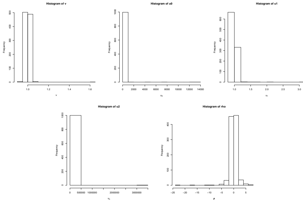
Figure 8: Posteriors
