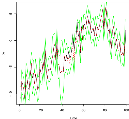
Figure 5: SIRS Algorithm
